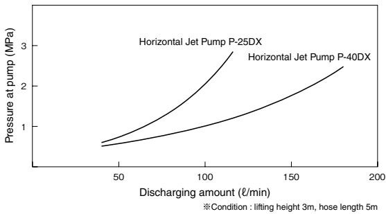
Horizontal Jet Pump performance curve
